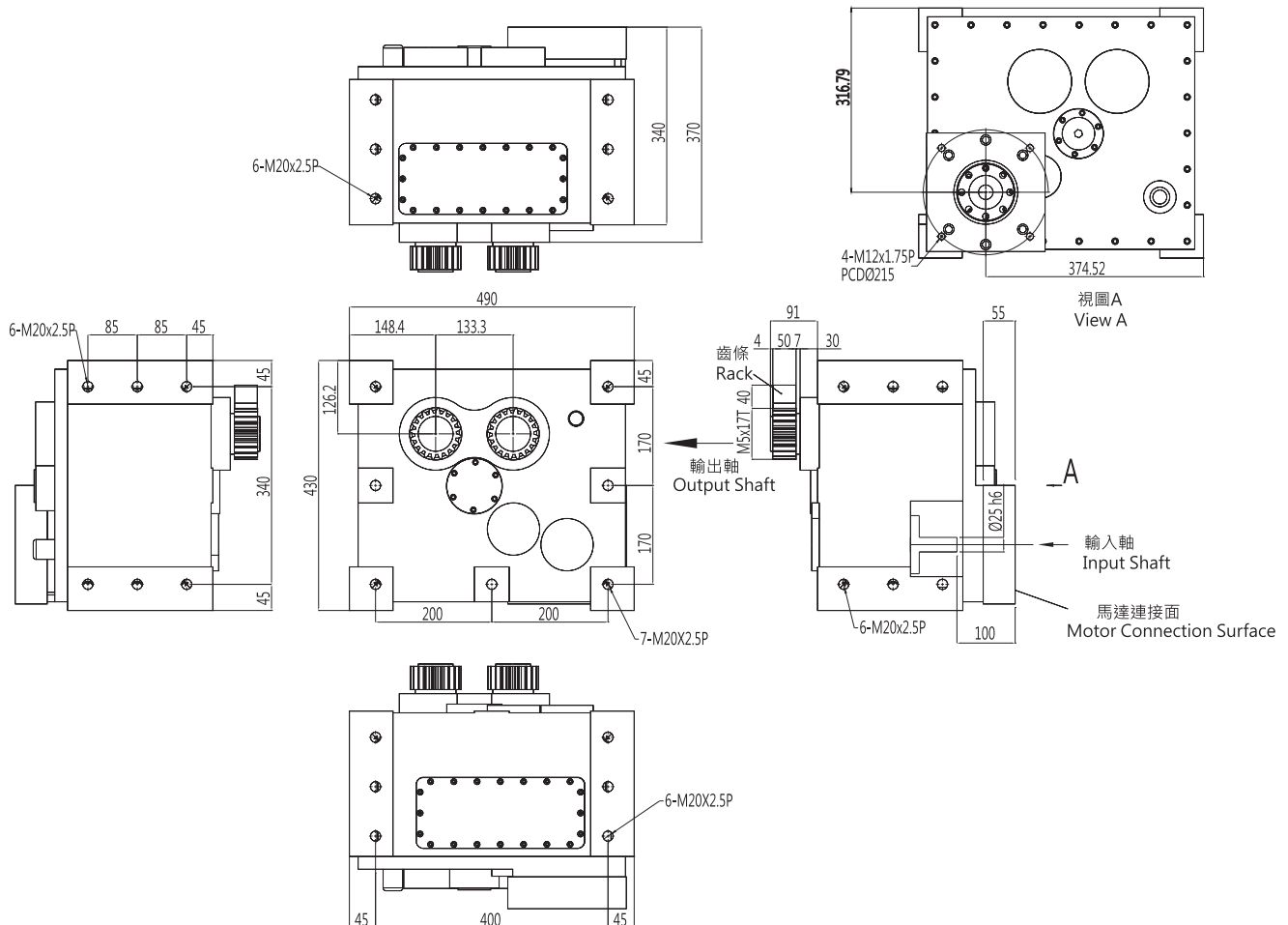
消隙減速機 Backlash Free Reducer SC-5FX
