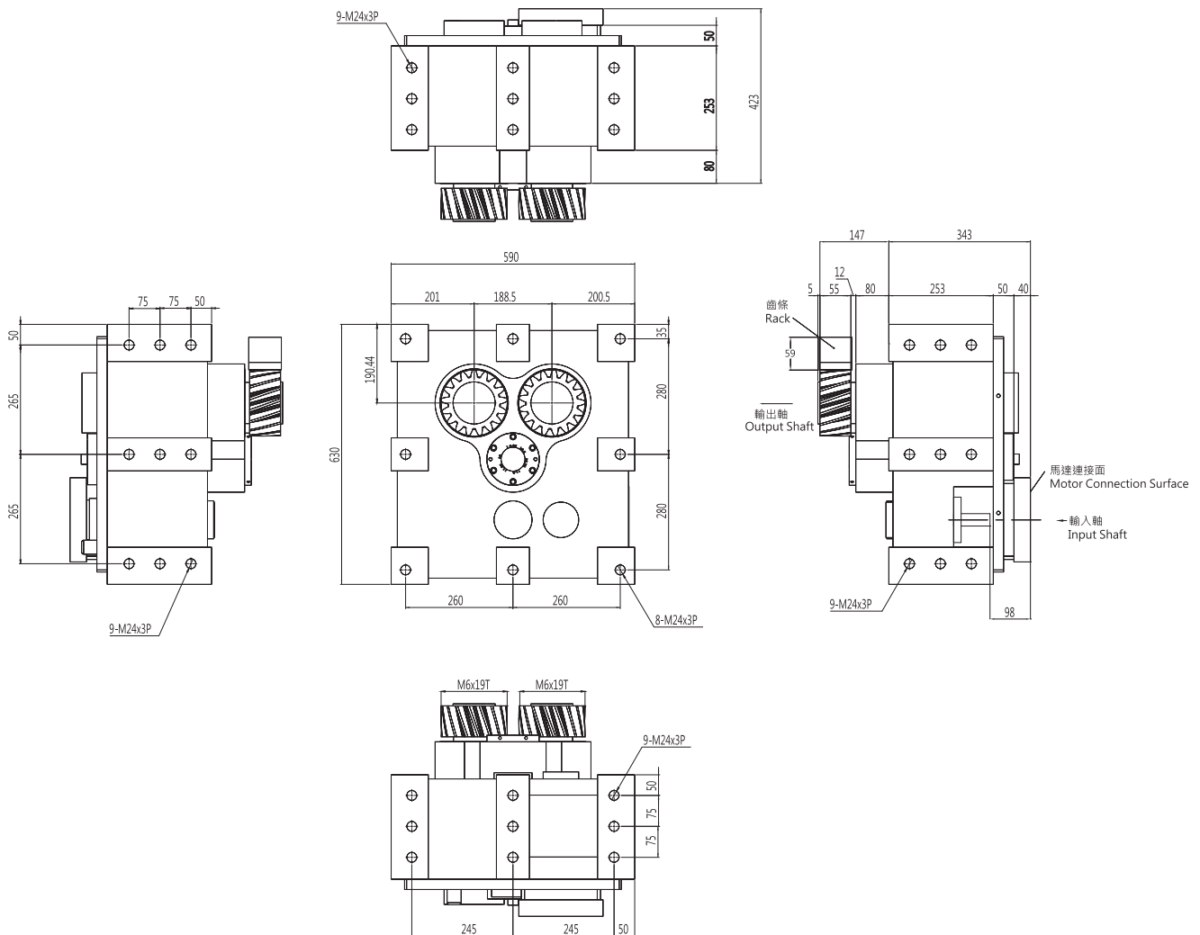
消隙減速機 Backlash Free Reducer SC-6FX
